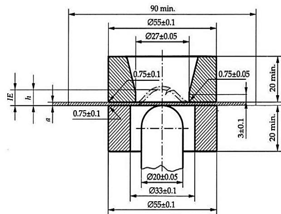
Fig. 6 Schematic of the Erickson test design used in this study in accordance with the standard ASTM E 643-84 [23].
