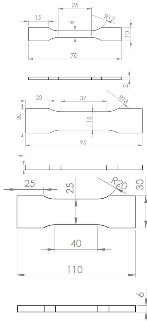
Fig. 2 The dimension of specimens prepared for tensile test.
