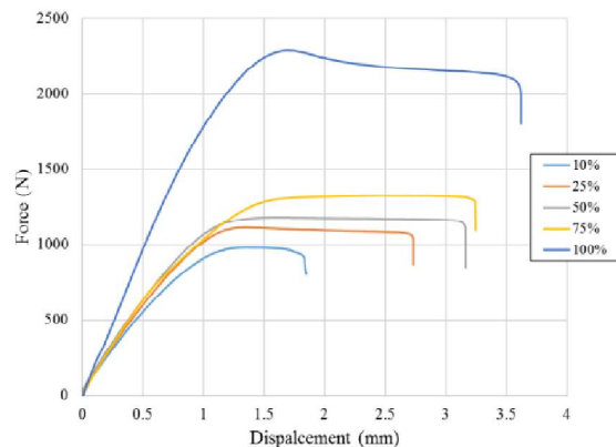
Fig. 10 Comparison of tensile force in specimens with different in-fill density.
