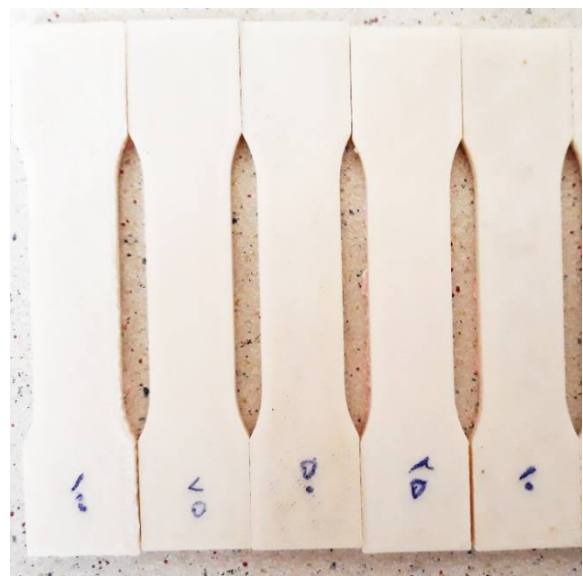
Fig. 3 The printed specimens with different in-fill density.
