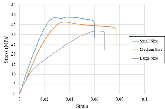
Fig. 9 Comparison of tensile stress in specimens with different size.
