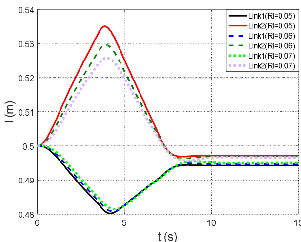
Fig. 9 The prismatic joints link's length variation
