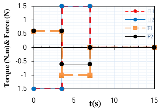
Fig. 4 The joints input torques and Forces
