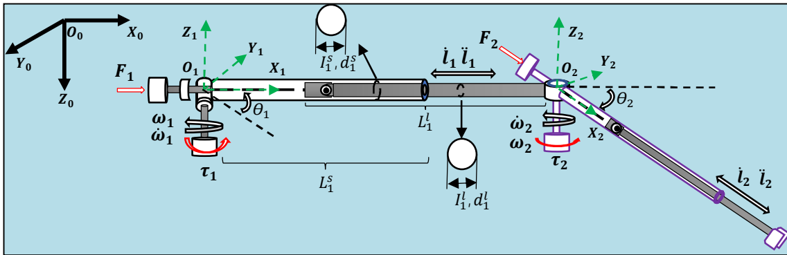
Fig. 3 Two-links manipulator with time variable structure in fluid medium
