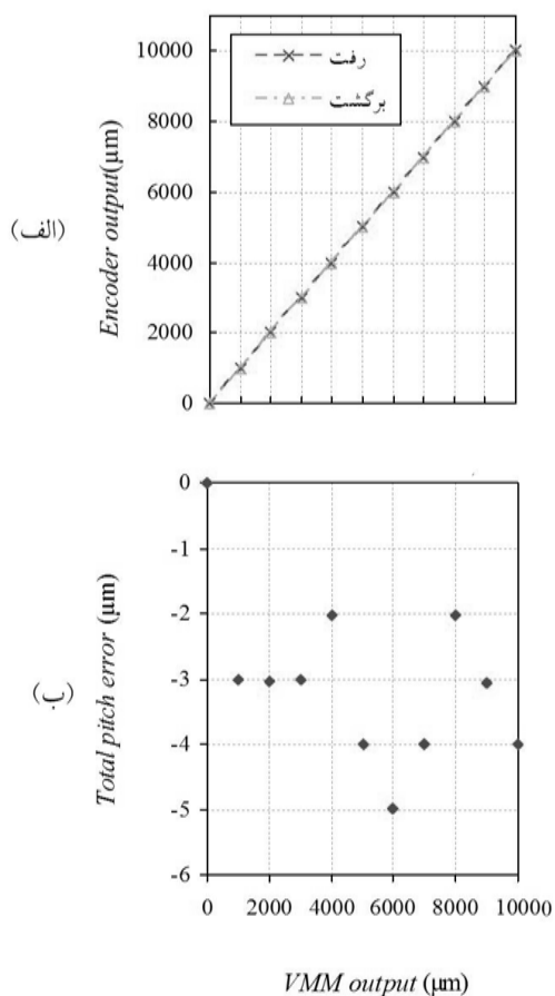
Fig. 17 (a) Calibration curve of encoder. (b) total pitch error for 30 μm gap
