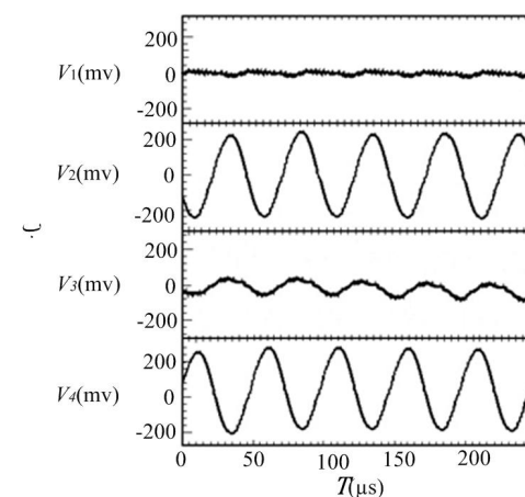
Fig. 13 Output signals of the four phase stator after one pitch movement of the slider over the stator
