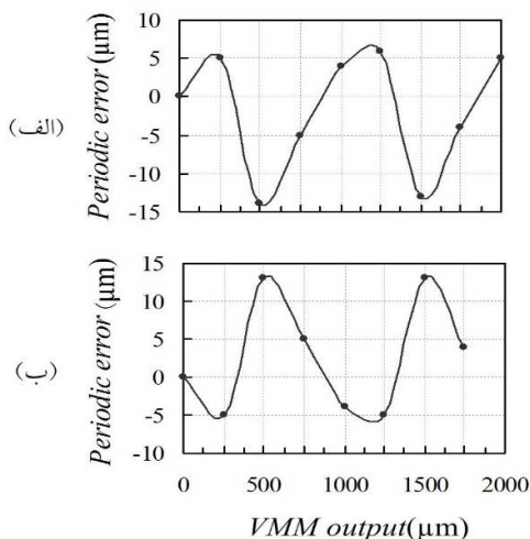
Fig. 18 Periodic error for 30 μm gap. (a) forward. (b) backward
