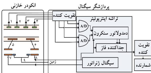
Fig. 9 Block diagram of signal processing for the encoder
