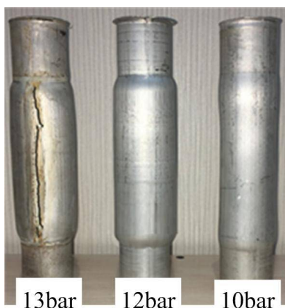
Fig. 8 Formed tubes under different initial gas pressure (ignition system I the middle of tube)
