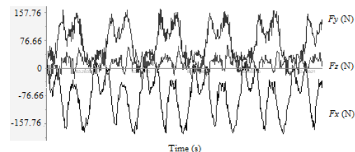
Fig. 4 A milling force graph in x, y, and z directions obtained by the dynamometer when n_s = 2000 rpm, f = 100 mm/min, a_p = 1 mm
