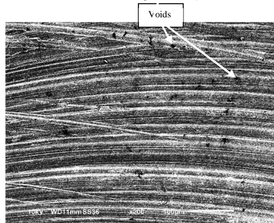
MQL with mineral oil, \times 200 (ج)
