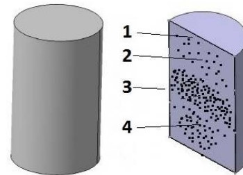
Fig. 8 Variation of density along the Al-20 vol% Al_2O_3 sample (compaction pressure of 450 MPa)
