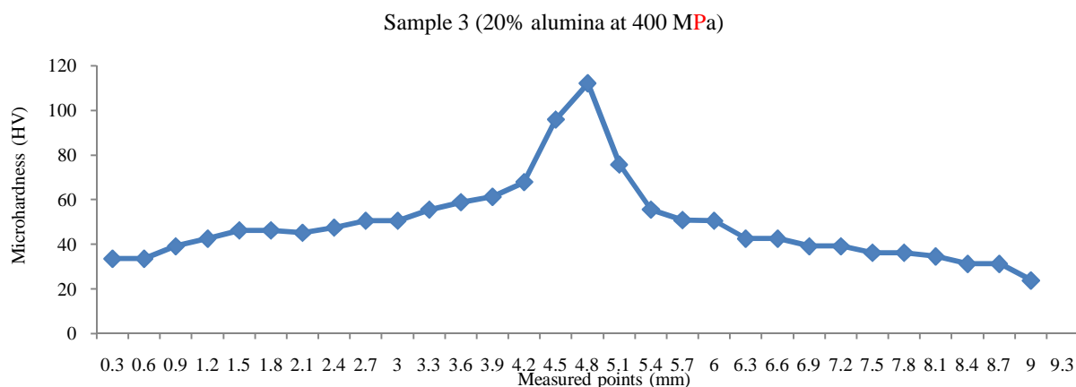
Fig. 16 Variation of micro-hardness along the cylindrical sample (Al-20 vol% alumina) under compacting pressure of 400 MPa
