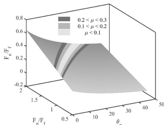
Fig. 5 Relation between finger forces, coefficient of friction of fingertip and angle between phalanges
