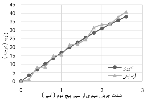
Fig. 10 Effect of change of current of second coil on encoder's angular position while first coil's current= 1.5A
