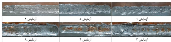
Fig. 9 Defective joints made with pinless tools
