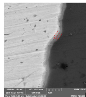
Fig. 15 Thin intermetallic layer created at the junction of aluminum and copper
