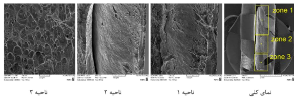
Fig. 16 SEM images of the failure surface of the tensile specimen
