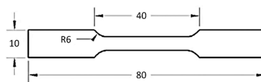
Fig. 2 Dimensions of the tensile test specimen (mm)
