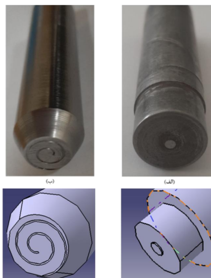
Fig. 1 Tools used for experiments: (a) pinned tool; (b) pinless tool
