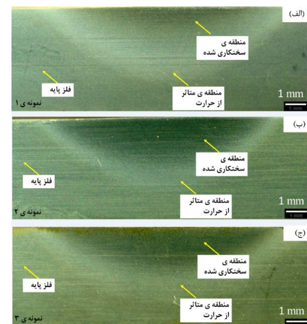
Fig. 2 Hardened area geometry for all three samples 1, 2 and 3
