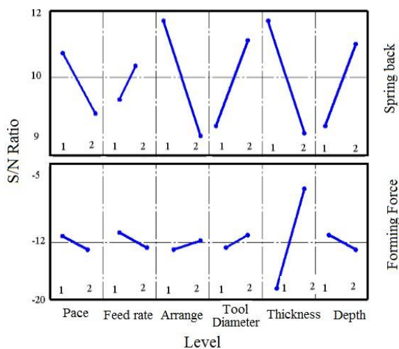
Fig. 10 S/N Diagram for springback and Forming Force
