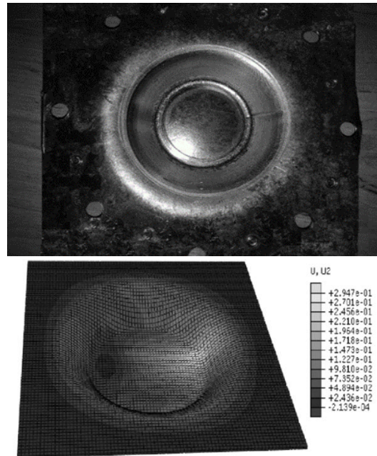
Fig. 7 View of the double layer sheet after practical and simulation (U2: displacement after springback (mm))
